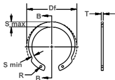
Free Diameter & Ring Measurements with Section B-B
