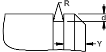
Exploded Groove Profile & Edge Margin (Y) Maximum bottom radii (R), .005 for ring sizes -62 thru -100; .010 for ring sizes -106 thru -400
