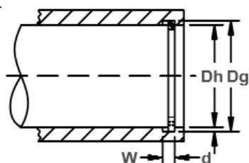
Housing Diameter & Groove Dimensions
